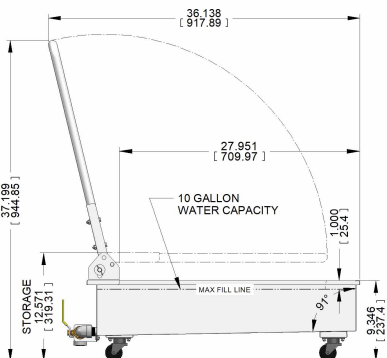
BOC-10 (10 gallon)
