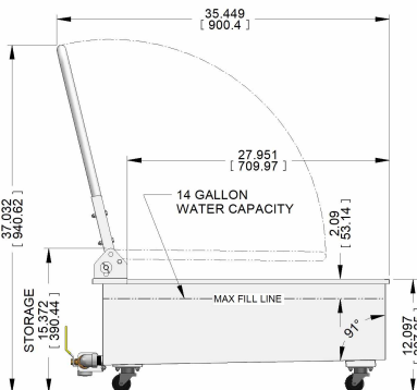
BOC-14 (14 gallon)
